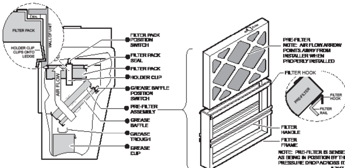
Fig. 7 Filter Installation
