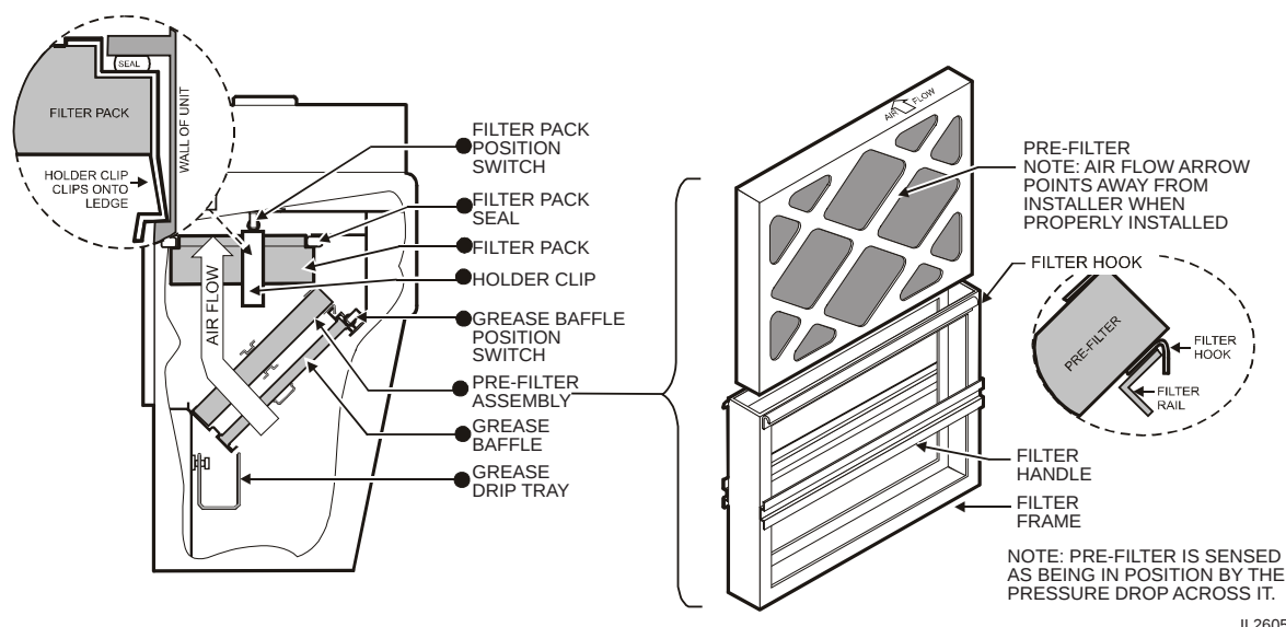
Fig. 6 Filter Installation
