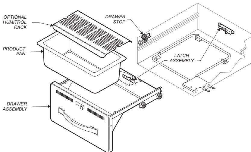
Fig. 9 Roll Warmer Drawer Pan Installation
