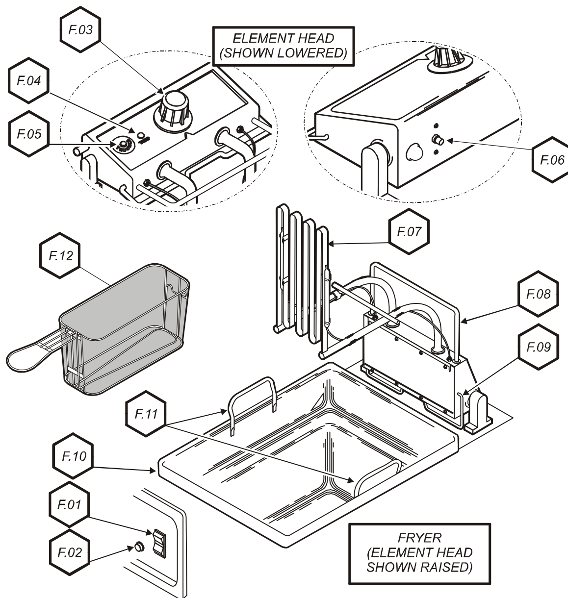
Fig. 3 Fryer Section
