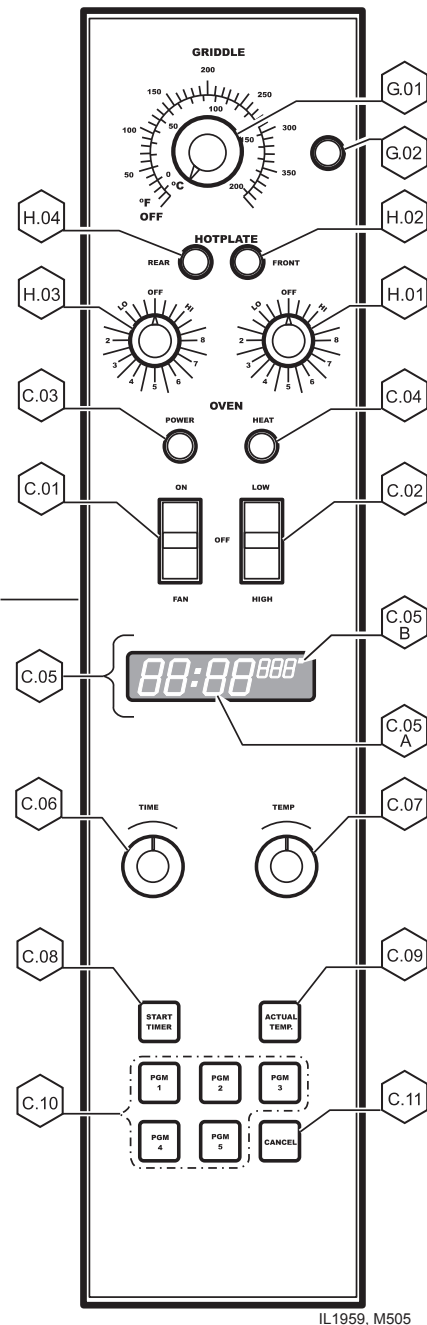
Fig. 4 Control Panel
