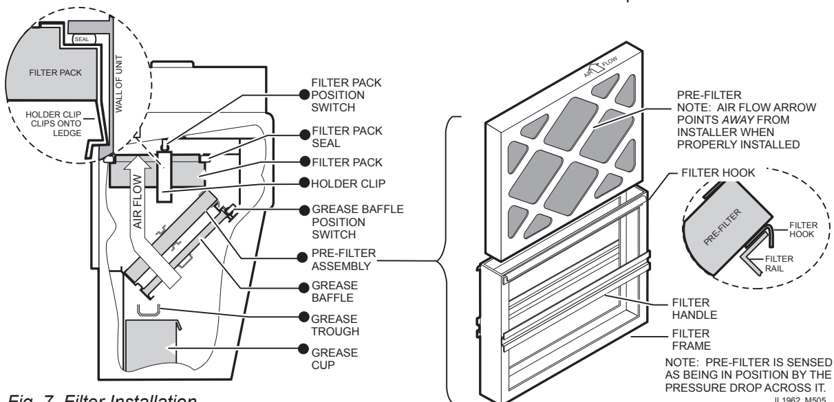
Fig. 7 Filter Installation
